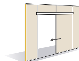
Doorway for single-panel face-mounted sliding door
